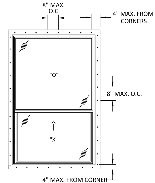
ANCHOR LAYOUT NAIL FIN INSTALLATION
