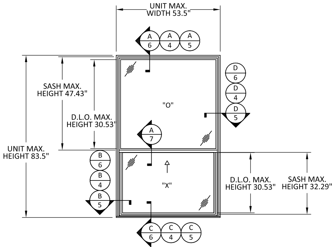
TYPICAL ELEVATION SINGLE HUNG ORIEL
