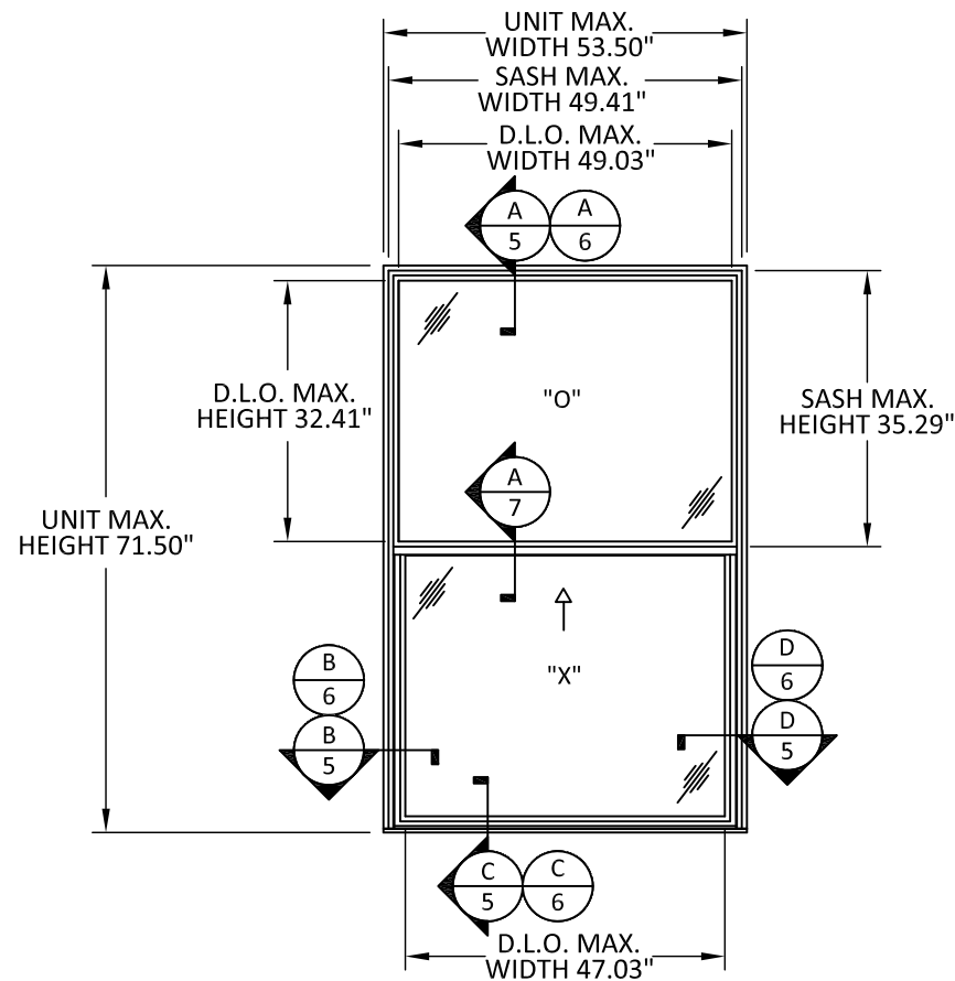
TYPICAL ELEVATION SINGLE HUNG EQUAL
