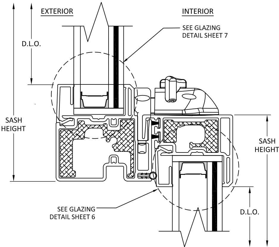
A 7 VERTICAL SECTION MEETING RAIL
