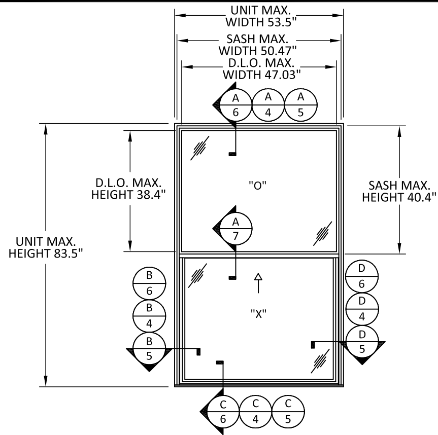
TYPICAL ELEVATION SINGLE HUNG EQUAL
